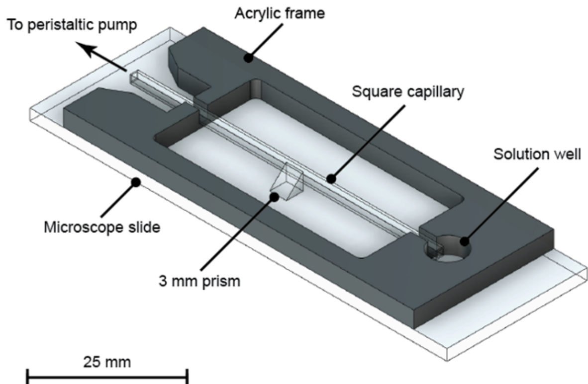
Figure S2. The acrylic bracket used to hold the square capillary tube containing a Chaoborus air-sac, related to Figures 1A-C and 3C-D and STAR Methods. Solutions placed in the solution well were drawn past the air-sac by a peristaltic pump. The subject was viewed from below using an inverted microscope. The second prism used to direct light horizontally through the capillary is not shown. This bracket was used to measure air-sac profile area as well as diameter as shown in Figure 1B and C. A similar device with four tubes and no prism was used to record air-sac profile areas shown in Figure 3C and D.
